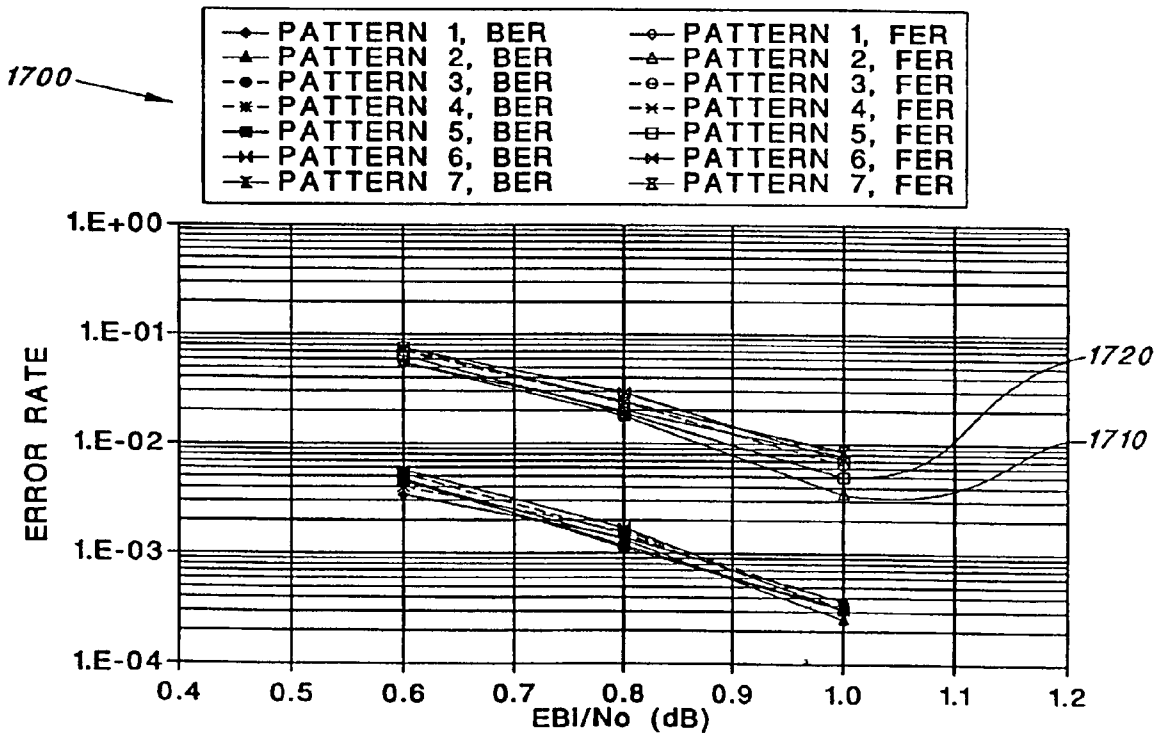
FIG. 17 COMPARISON OF RATE 1/3 PUNCTURING SCHEMES, FRAME=512
