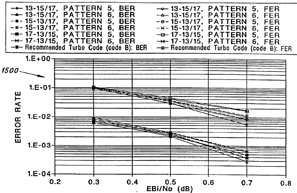
FIG. 15 COMPARISON AGAINST OTHER PUNCTURING SCHEMES, FRAME=512
