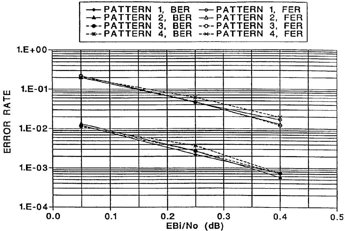
FIG. 13 BER/FER PERFORMANCE OF CODE #1, FRAME SIZE=1024
