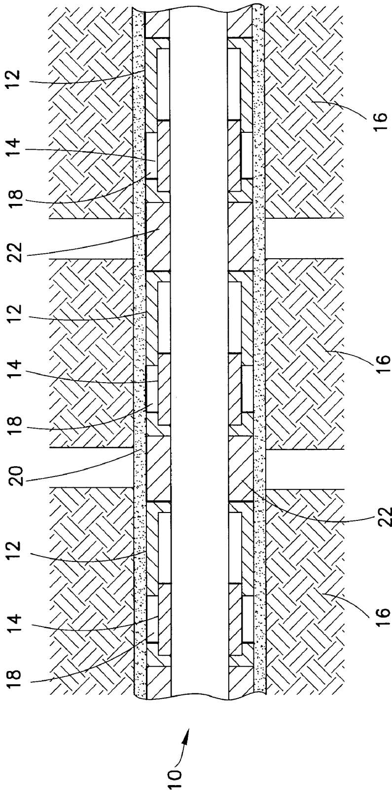
FIG. 1 PRIOR ART
