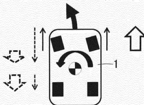
Fig. 13C CASE OF REAR-WHEEL DRIVE VEHICLE (YAW MOMENT CONTROL BY FRICTION BRAKE)
