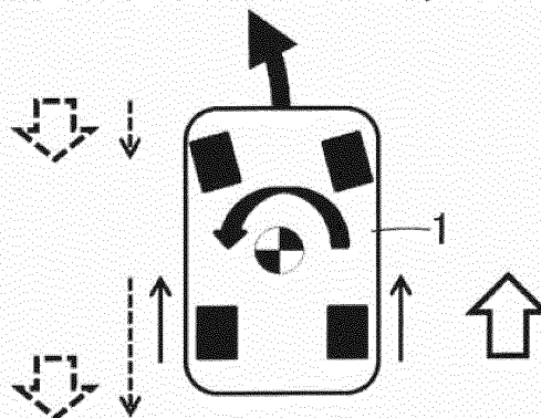
Fig. 13C CASE OF REAR-WHEEL DRIVE VEHICLE (YAW MOMENT CONTROL BY FRICTION BRAKE)
