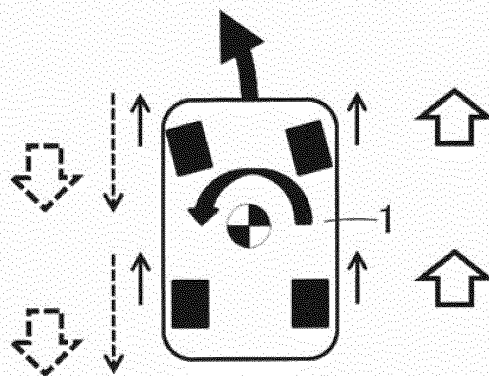
Fig. 13B CASE OF FRONT-WHEEL DRIVE VEHICLE (YAW MOMENT CONTROL BY FRICTION BRAKE)
