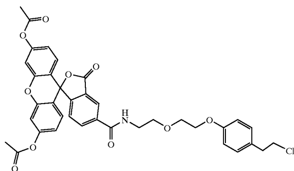
a compound of formula XXXII
