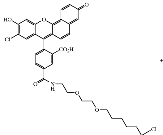
a compound of formula XVII
