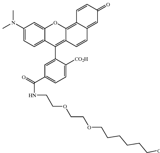
a compound of formula XX
