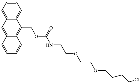
a compound of formula XXV
