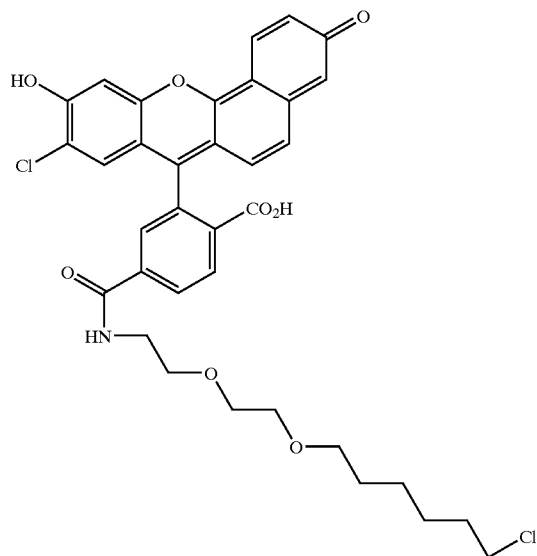
a compound of formula XVIII
