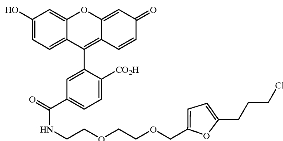
a compound of formula XXXIV
