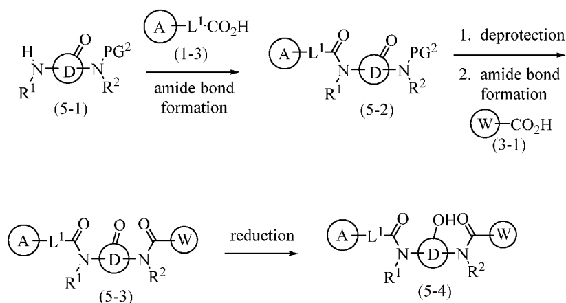
Scheme 5B: Representative scheme for synthesis of exemplary compounds of the invention
