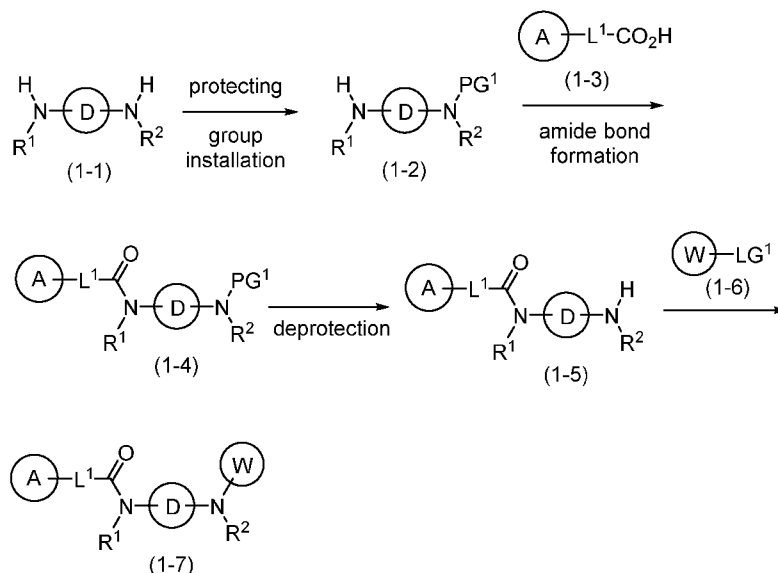
Scheme 1: Representative scheme for synthesis of exemplary compounds of the invention.
