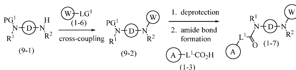
Scheme 9: Representative scheme for synthesis of exemplary compounds of the invention
