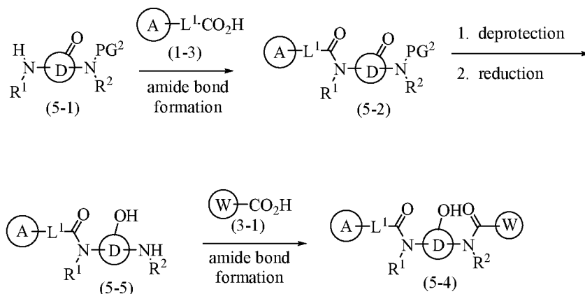
Scheme 5B: Representative scheme for synthesis of exemplary compounds of the invention
