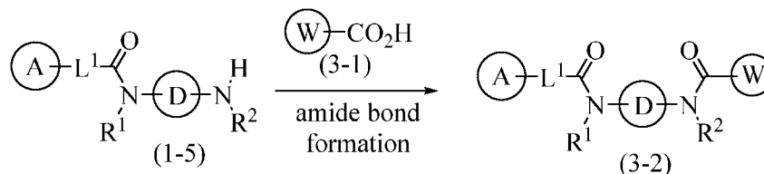
Scheme 3: Representative scheme for synthesis of exemplary compounds of the invention
