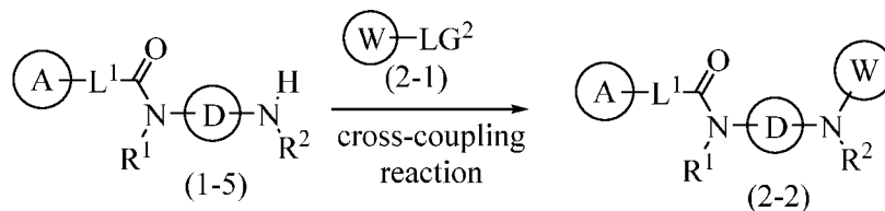
Scheme 2: Representative scheme for synthesis of exemplary compounds of the invention
