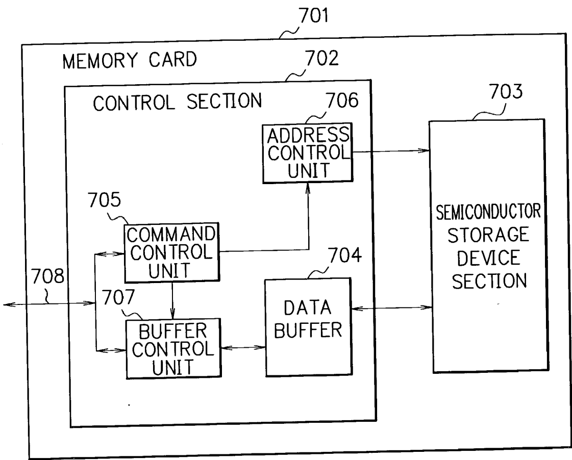
FIG. 7 PRIOR ART
