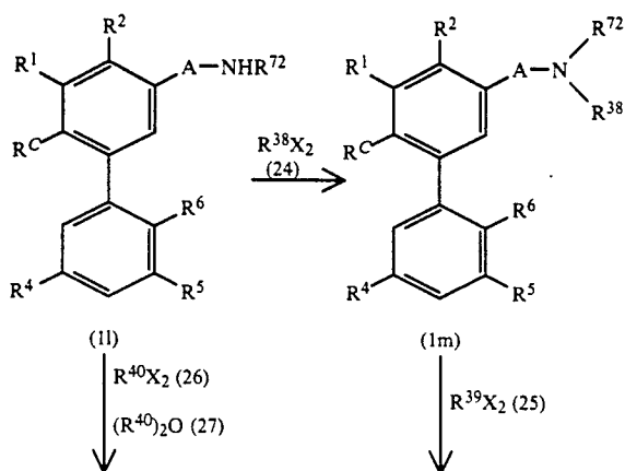
Reaction formula-13
