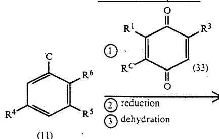
Reaction formula-17
