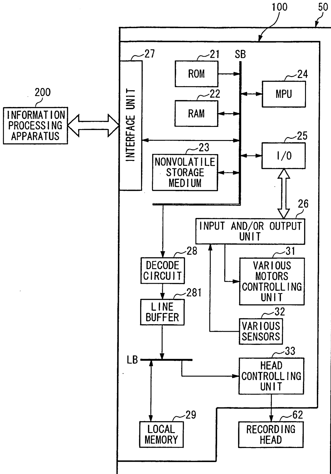
INKJET TYPE RECORDING APPARATUS
