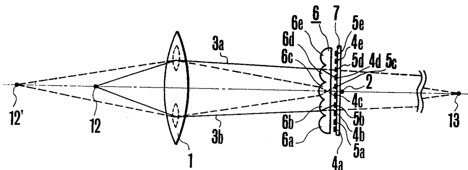
FIG. 2 (PRIOR ART)
