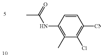
1C. 3-Chloro-4-cyano-2-methylphenylacetamide
