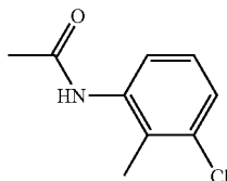
1A. 3-Chloro-2-methylphenylacetamide
