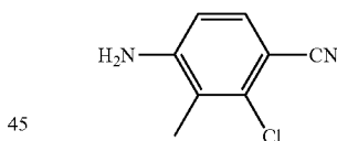
1D. 3-Chloro-4-cyano-2-methylphenylaniline
