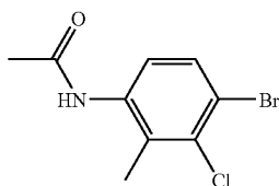
1B. 4-Bromo-3-chloro-2-methylphenylacetamide
