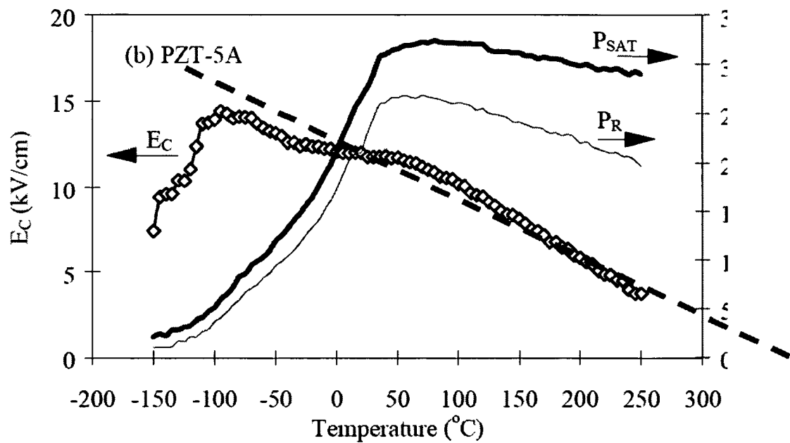
Figure 9. The coercive field necessary to pole and repole PZT ferroelectric ceramic decreases linearly with temperature 13 .
