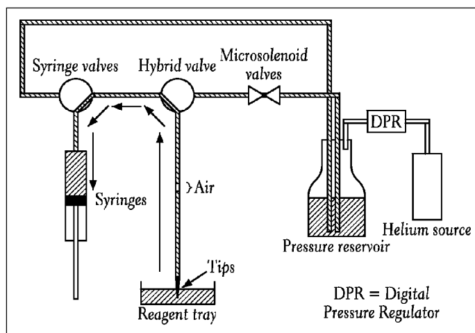
Reagent Aspiration, using the Syringe Path
