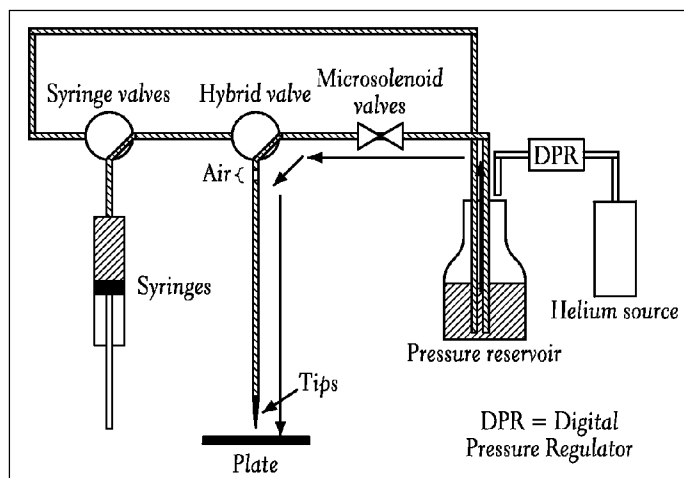
Reagent Dispense, using the Pressure Path
