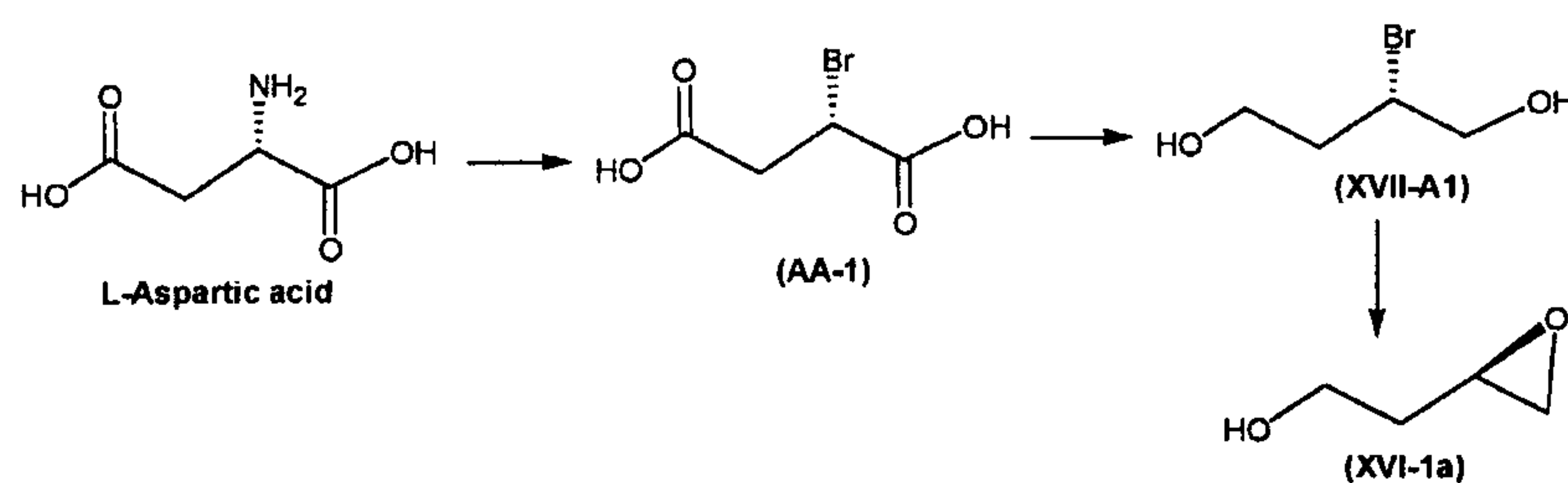
Scheme A2-1. Preparation of enantiopure epoxide from L-aspartic acid.
