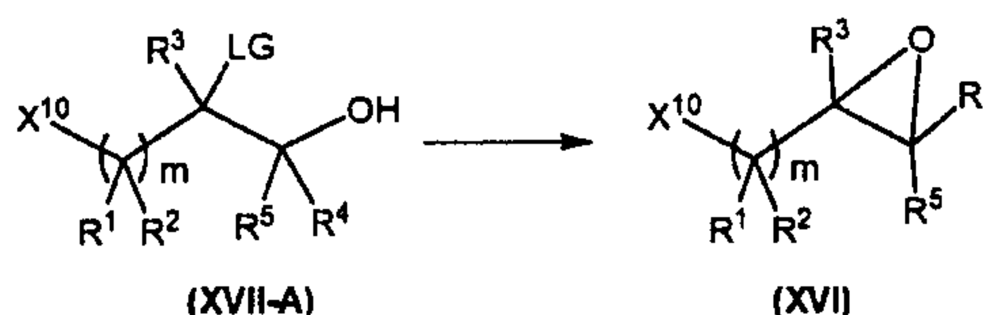
Scheme A2. Epoxidation via leaving group displacement.
