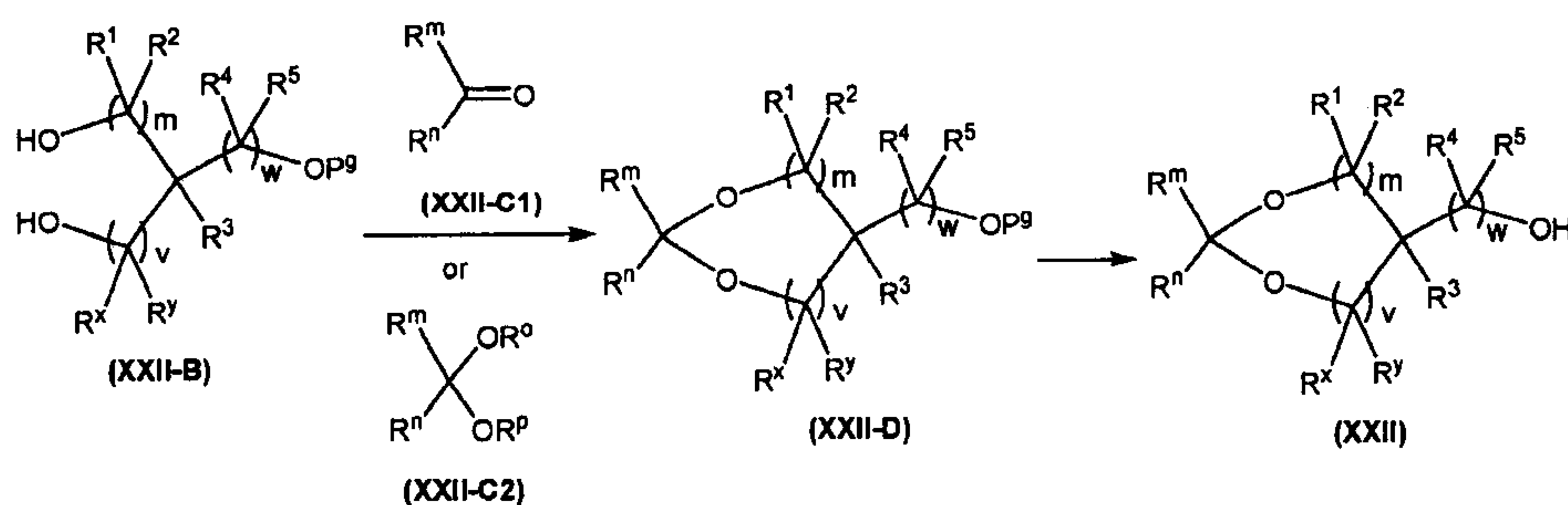
Scheme B1-1. Preparation of compounds of formula (XXII).
