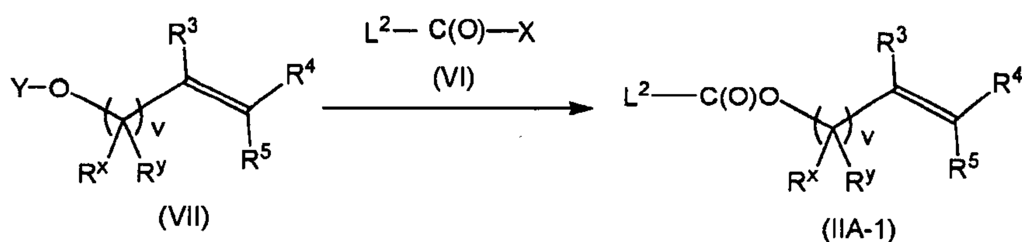
Scheme C2. Preparation of compounds of the formula (IIA-1).
