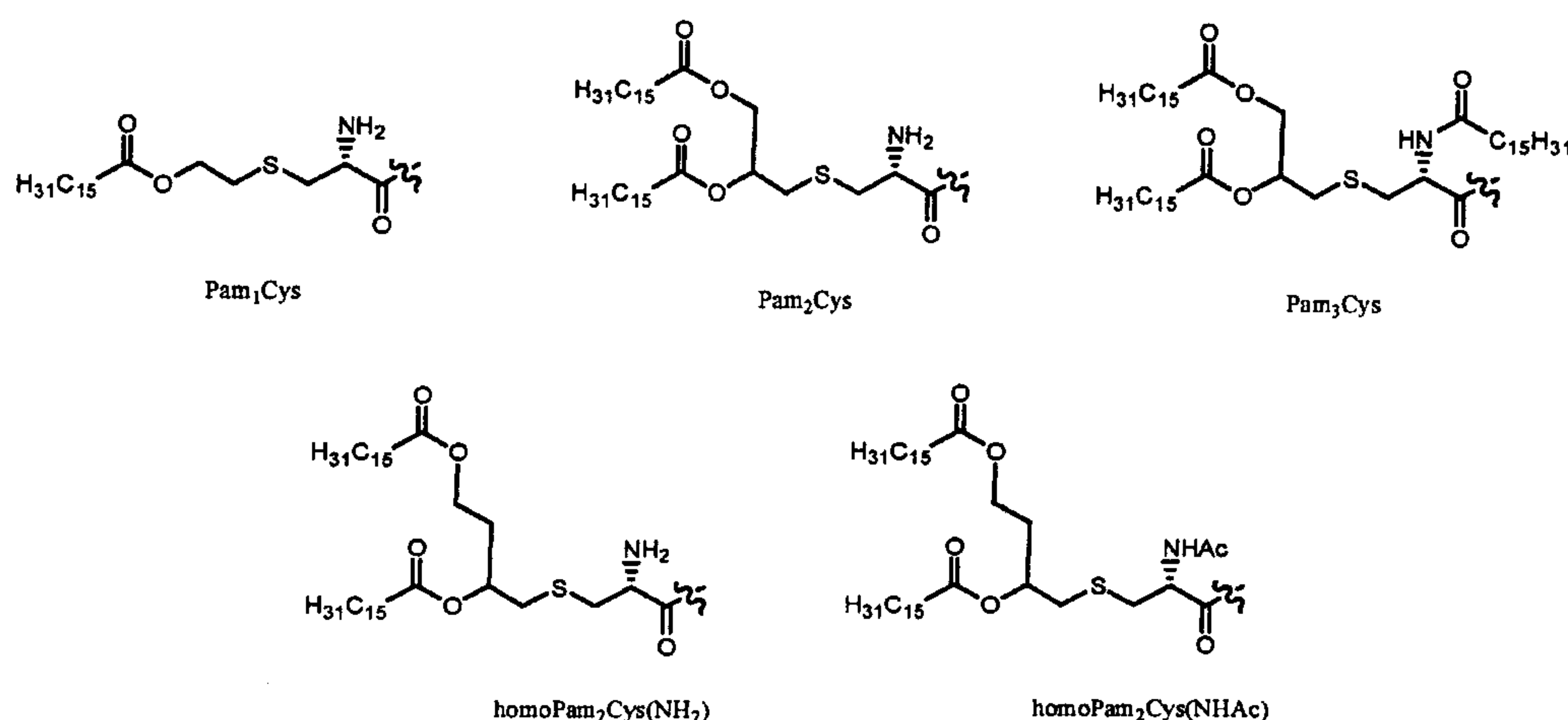
Scheme 3A. Structures of Pam1Cys, Pam2Cys, Pam3Cys, homoPam2Cys(NH 2 ) and homoPam2Cys(NHAc) referred to in Table 2.
