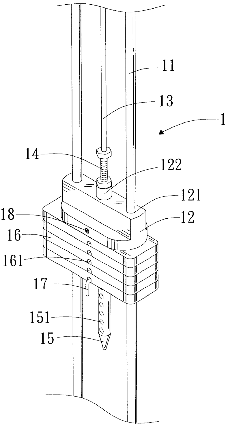
FIG.1 Prior Art
