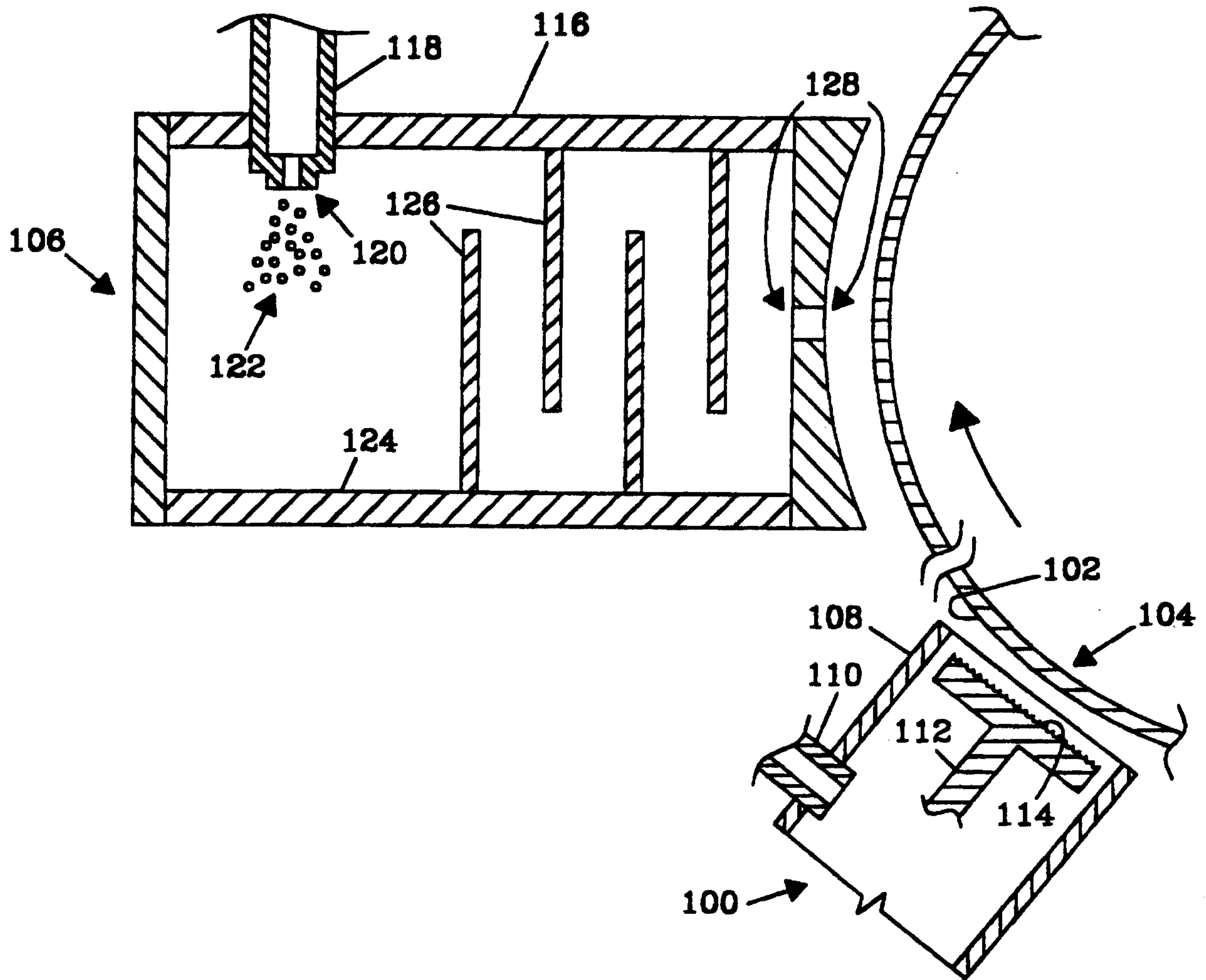
Fig. 1a (PRIOR ART)
