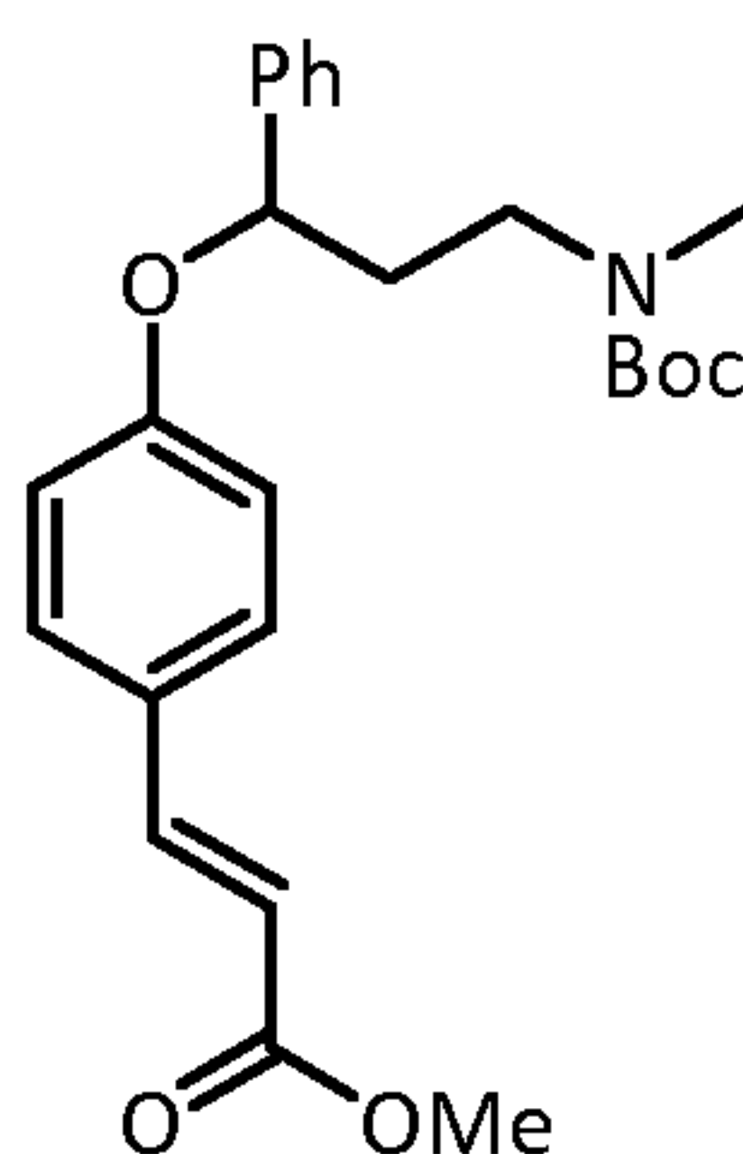
(E)-Methyl 3-[4-[3-[ tert -butoxycarbonyl(methyl)amino]-1-phenylpropoxy]phenyl]acrylate
