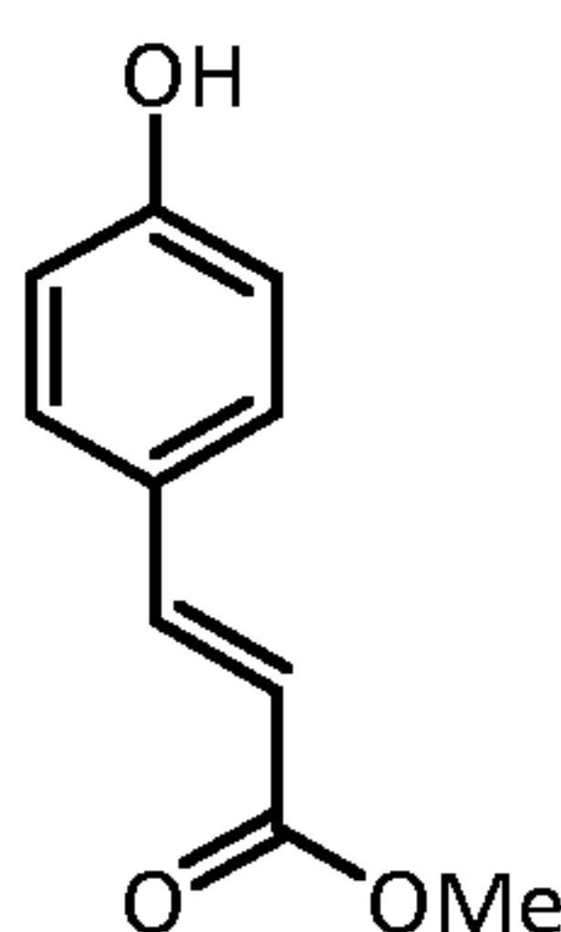
(E)-Methyl 3-(4-hydroxyphenyl)acrylate
