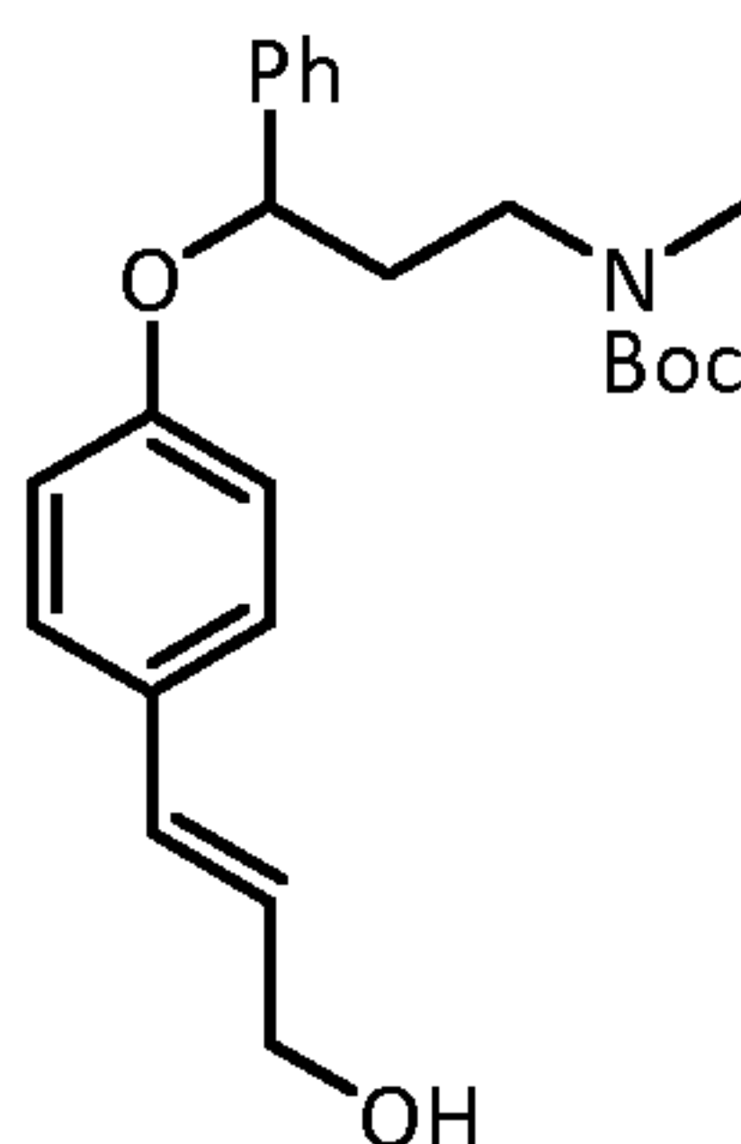
(E)-Methyl 3-(4-hydroxyphenyl)acrylate
