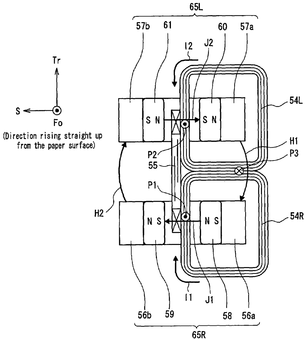
FIG. 7 PRIOR ART
