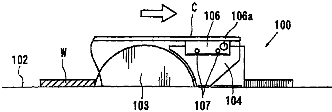
FIG. 51 PRIOR ART
