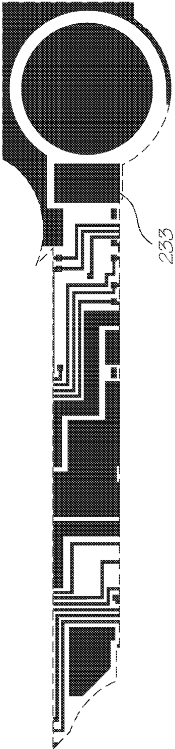
Metal 2 mask
