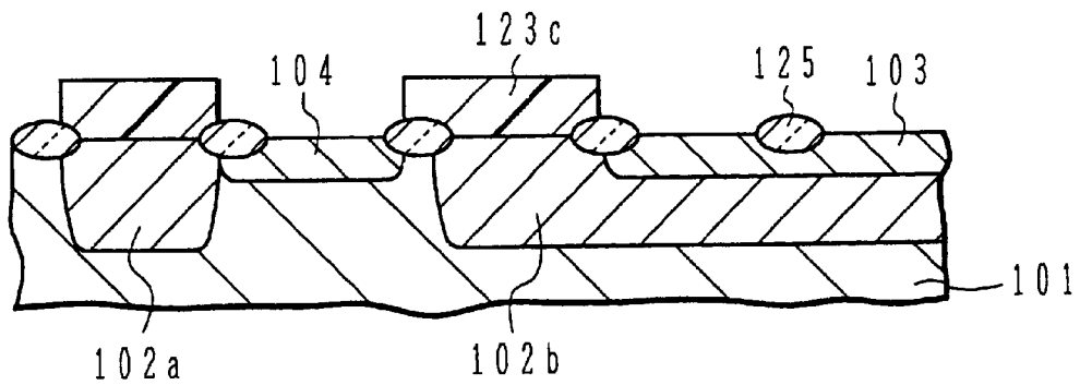
FIG.10C PRIOR ART
