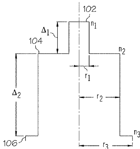
INDEX OF REFRACTION PROFILE
