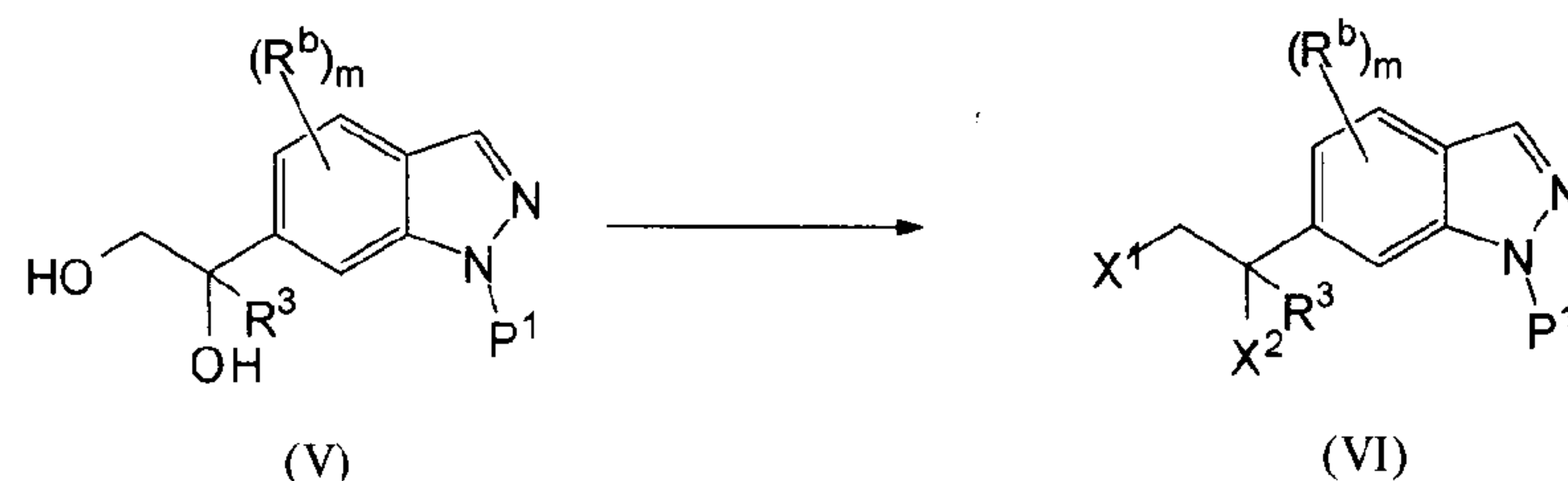
reaction 4
