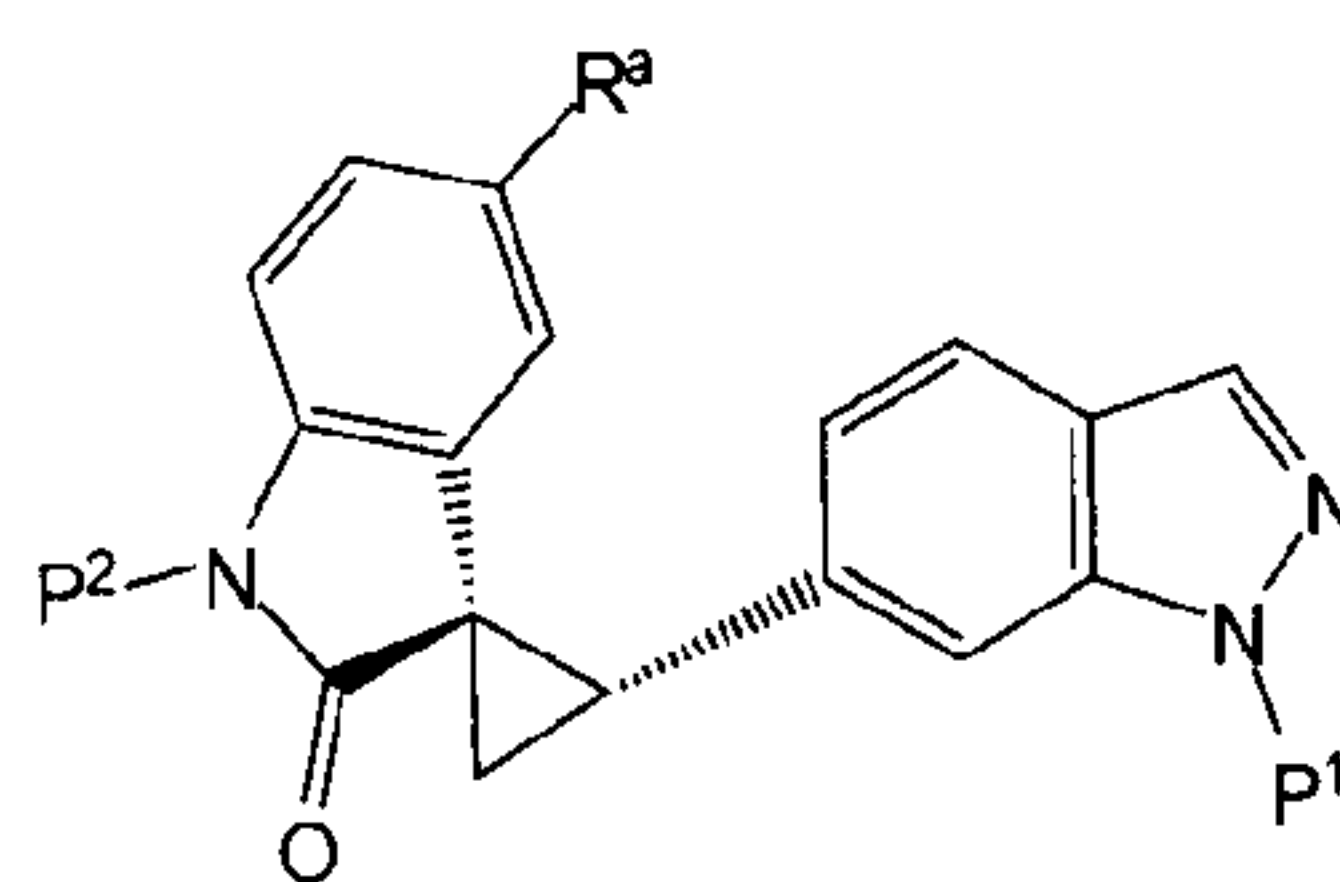
(XIb)
