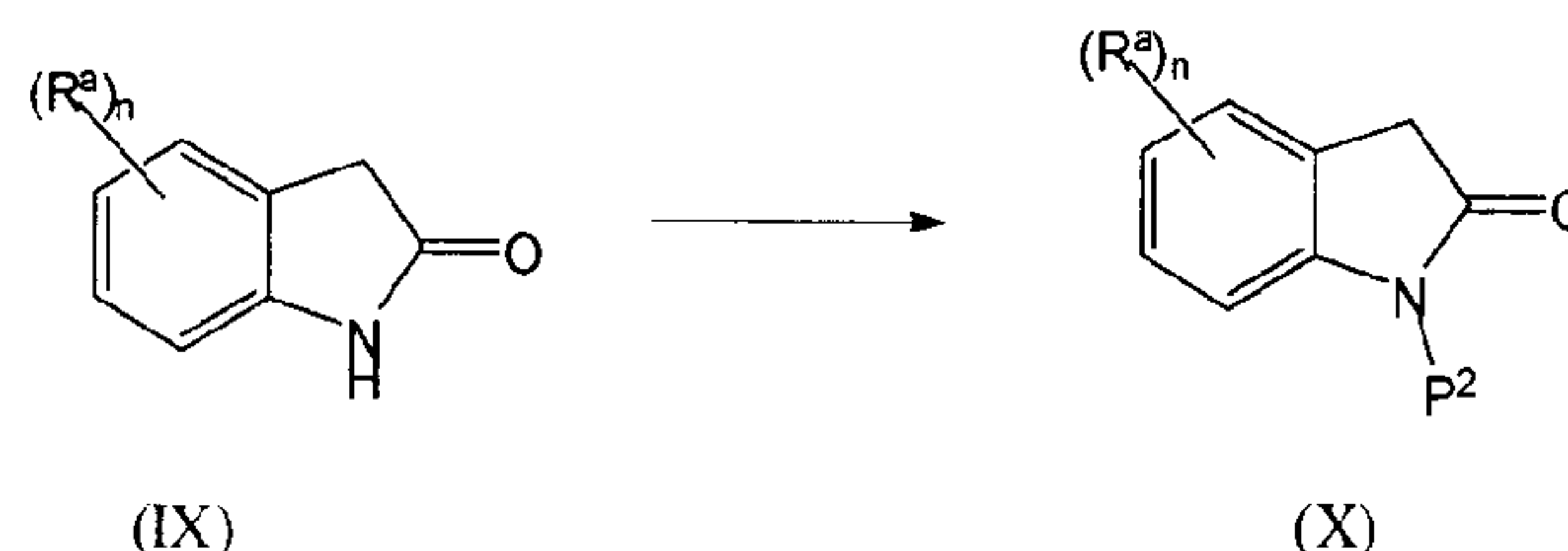
reaction 6
