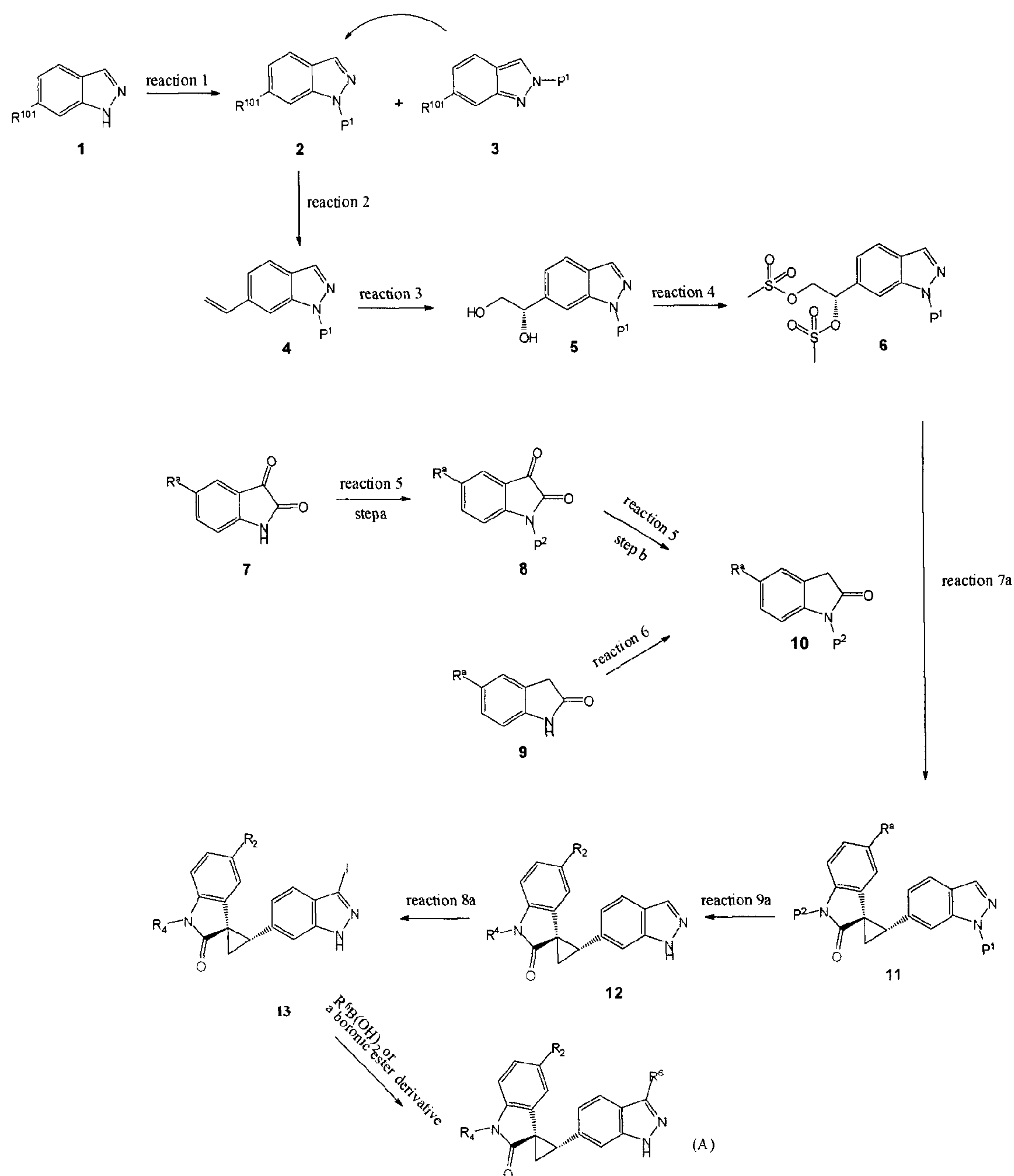
Scheme 1
