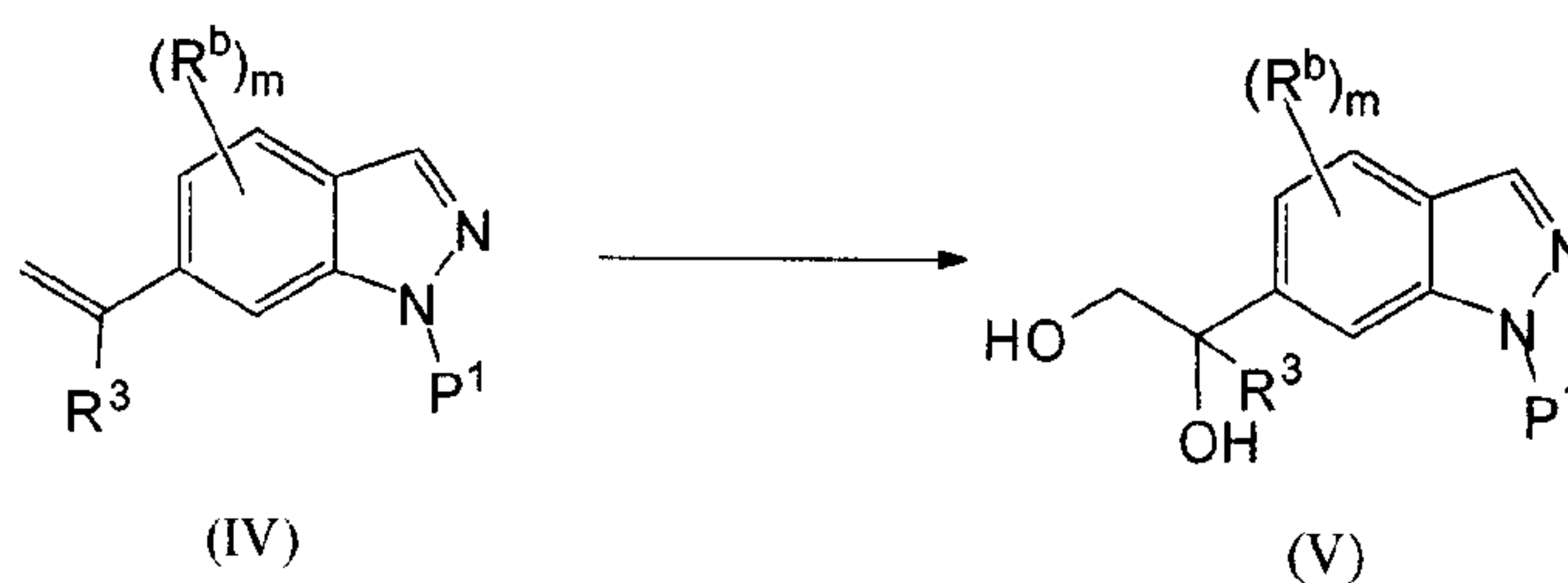
reaction 3
