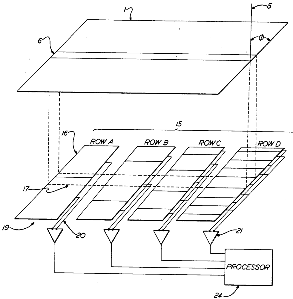
FIG. 1 PRIOR ART
