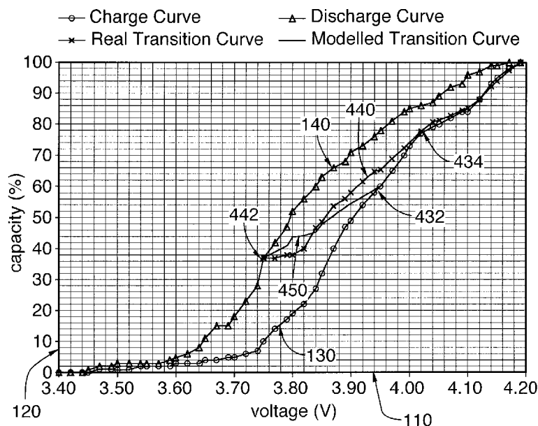
Discharge/Charge/Transition Curves
