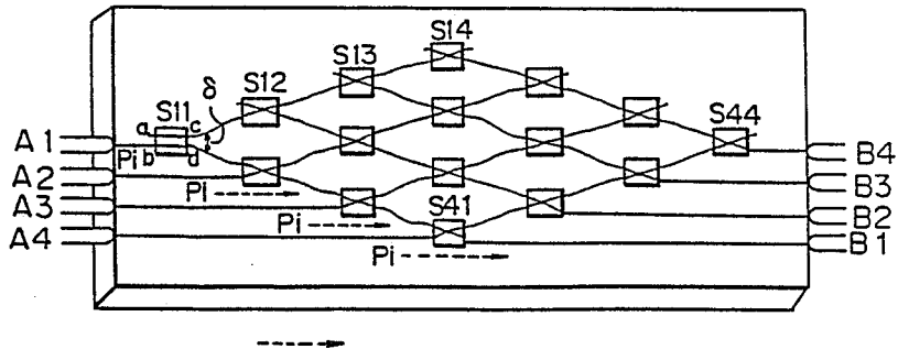
Fig. 4 PRIOR ART
