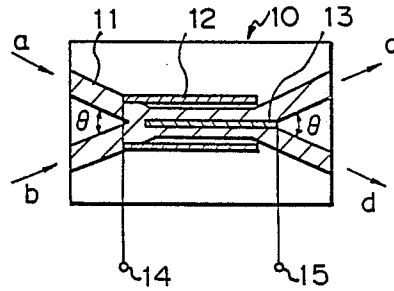
Fig. 4 PRIOR ART
