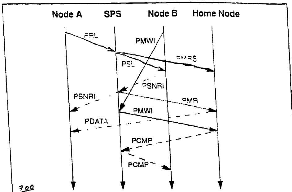
Figure 7 Timing Diagram for the Read-Write Conflict Problem
