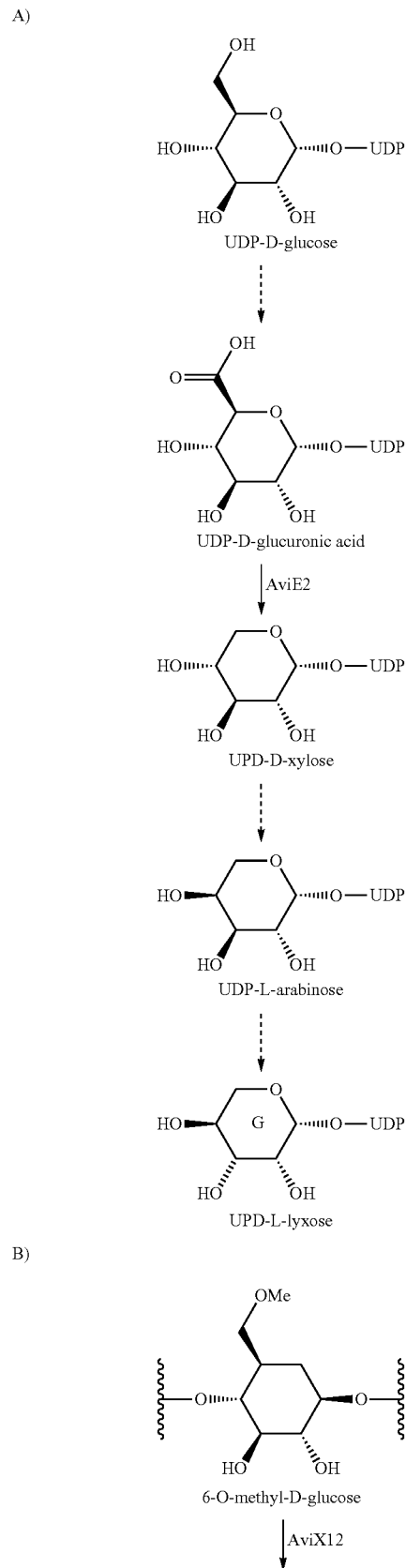
Scheme 1: Orthosomycin biosynthesis
