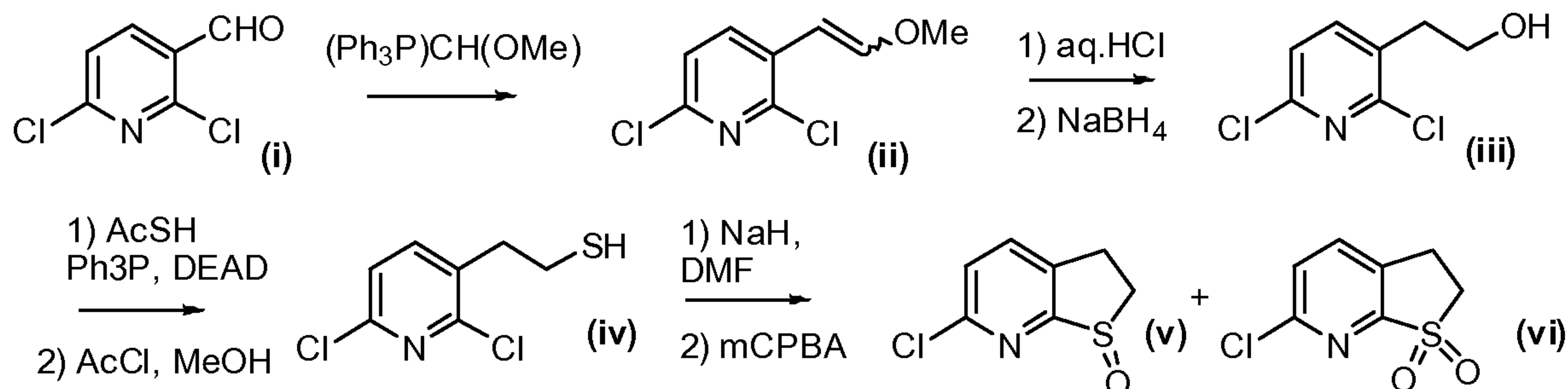
Scheme IV
