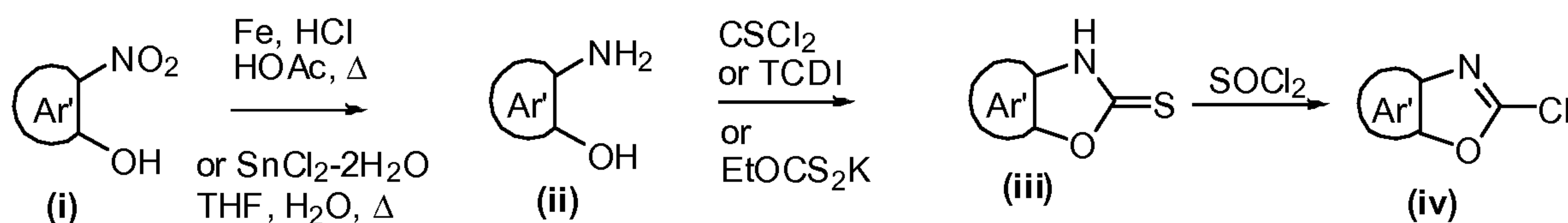
Scheme V
