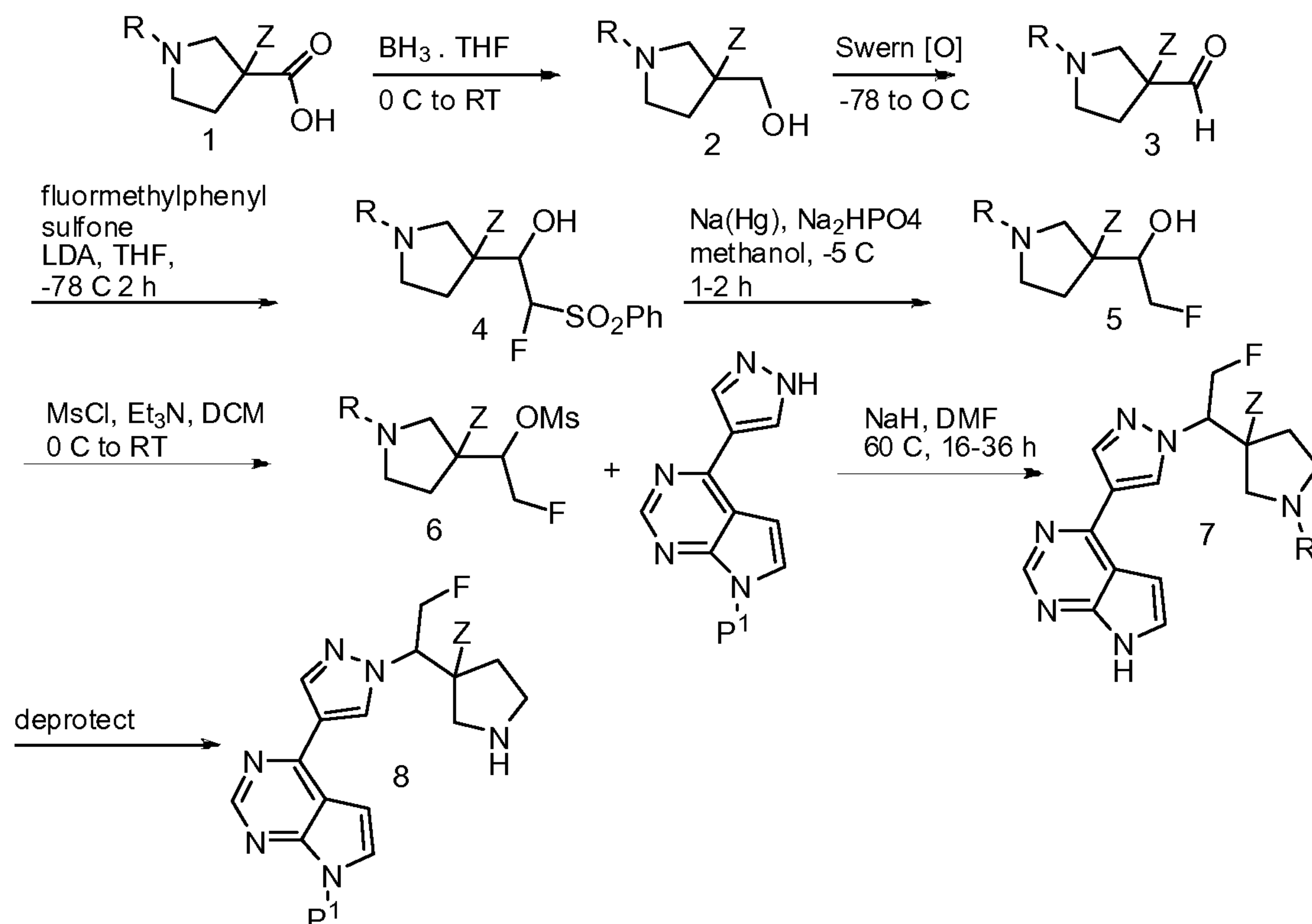
Scheme VIII
