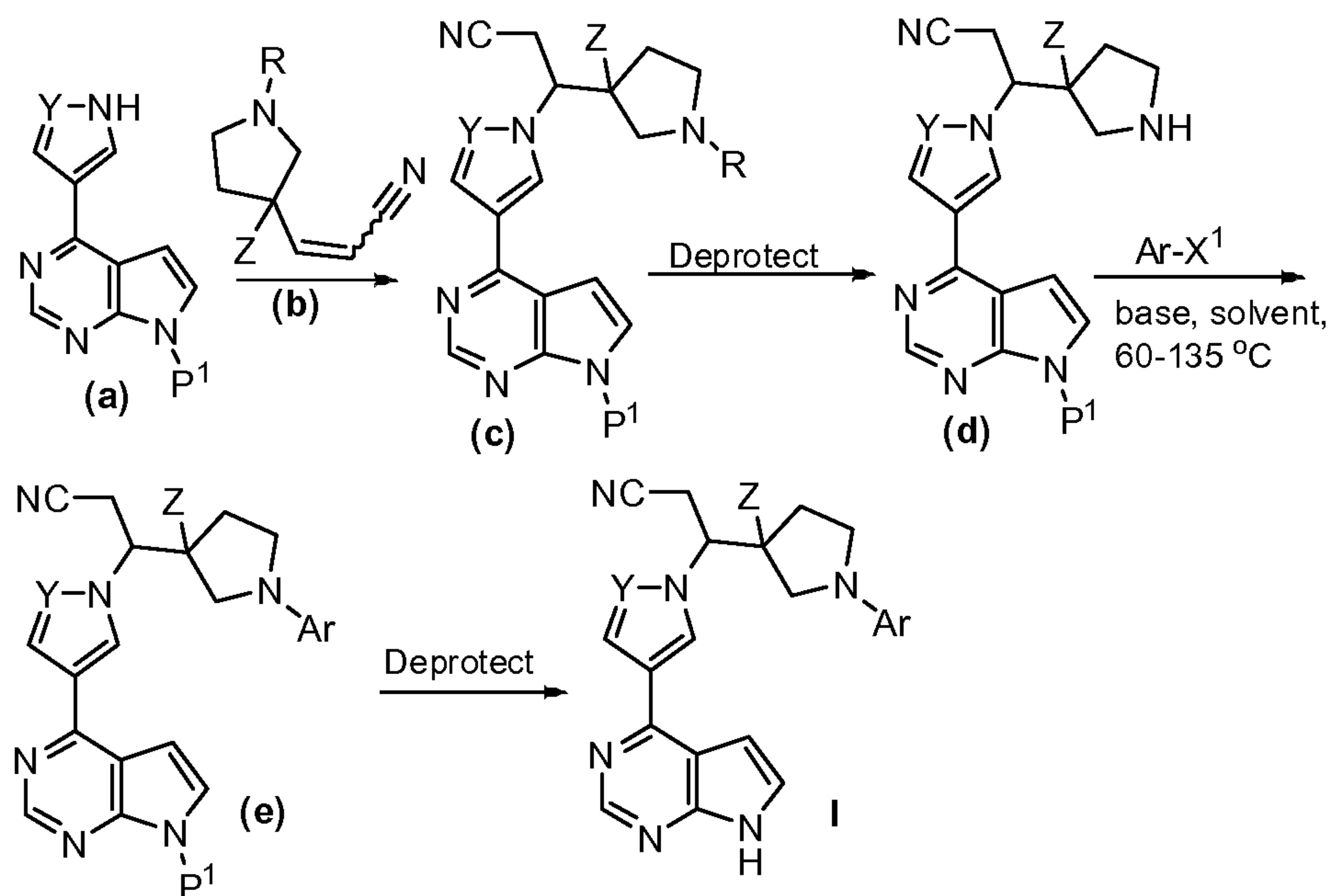
Scheme I
