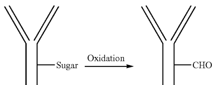
Scheme 4
