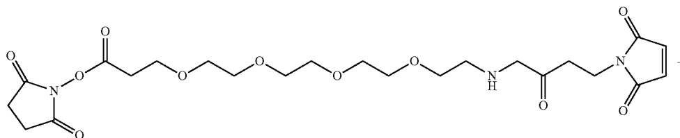
Scheme 7
