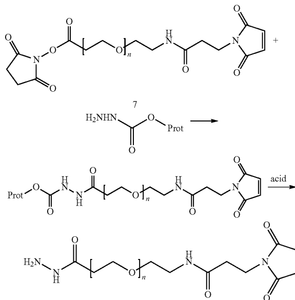
Scheme 6
