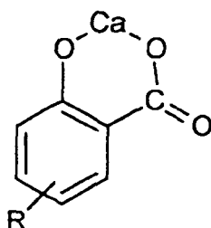
10 Compound A
