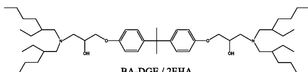
BA-DGE / 2EHA Mol. Wt. = 823.33
