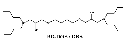
BD-DGE / DBA Mol. Wt. = 460.73
