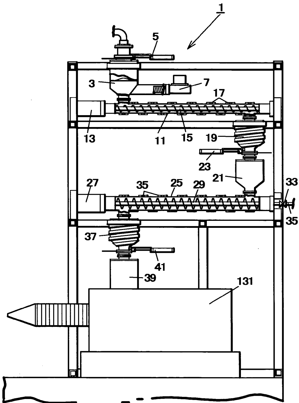
molding machine
