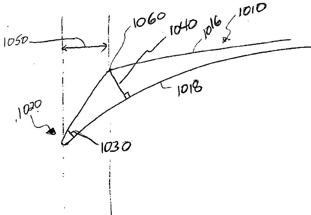
Figure 5: Prior Art
