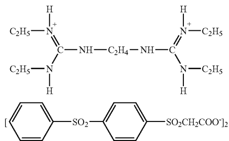
Base precursor compound-1
