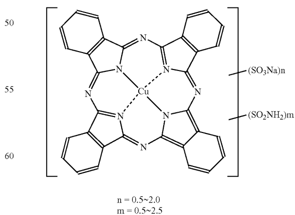
Blue dye compound-2
