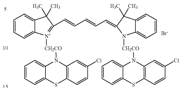
Cyanine dye Compound-1
