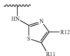
2-(1,3-THIAZOYL) RING SUBSTITUTION
