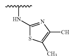
2-(4,5-DIMETHYL-1,3-THIAZOYL) GROUP
