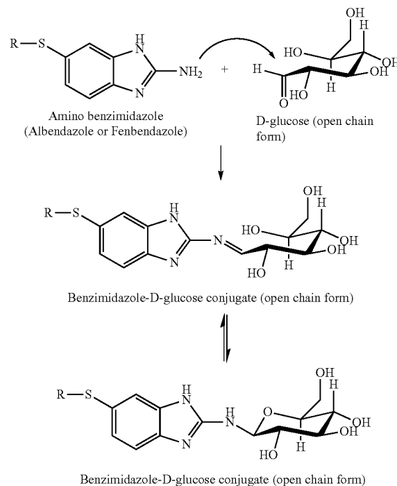
[Reaction Scheme 1]
