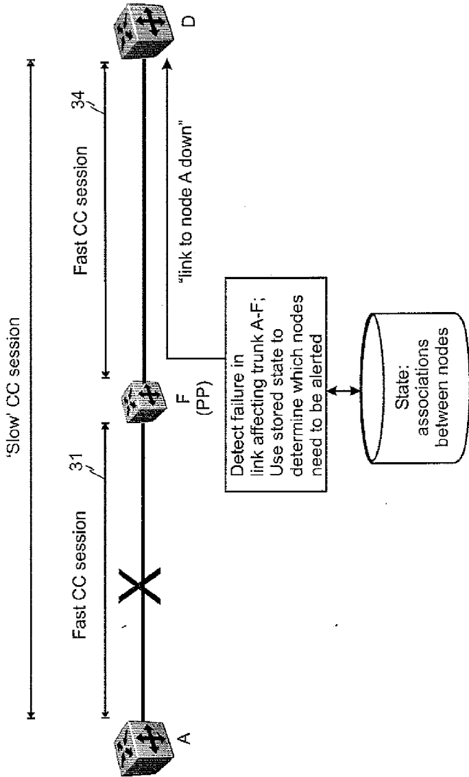
Trunk A-D routed via Pinning Point (PP) F Failure on leg A-F
