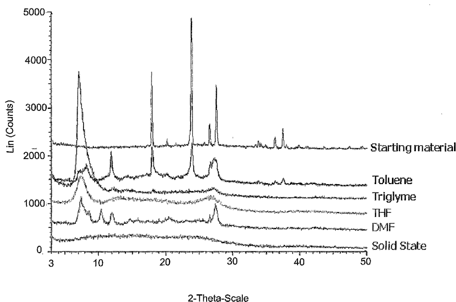
Powder X-ray diffraction patterns of polymerization products.
