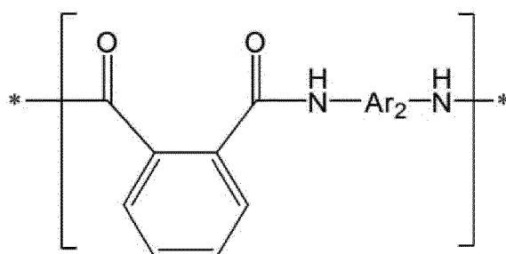
[Chemical Formula 2-2]
