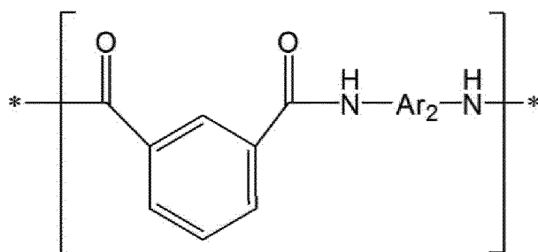
[Chemical Formula 2-1]
