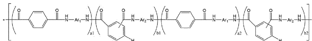
[Chemical Formula 4]
