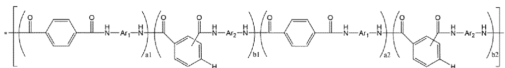
[Chemical Formula 4]
