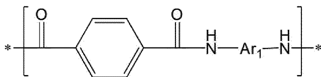
[Chemical Formula 1]
