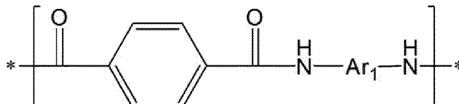
[Chemical Formula 1]
