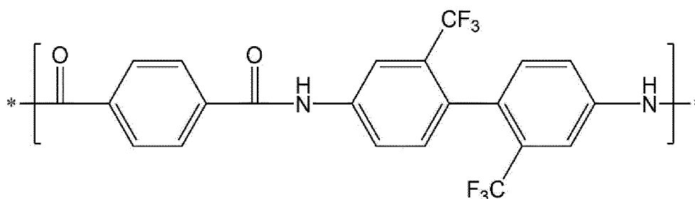
[Chemical Formula 1-1]
