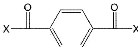
[Chemical formula 7]
