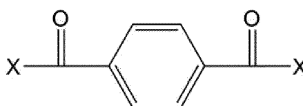
[Chemical formula 7]
