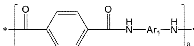
[Chemical Formula 5]
