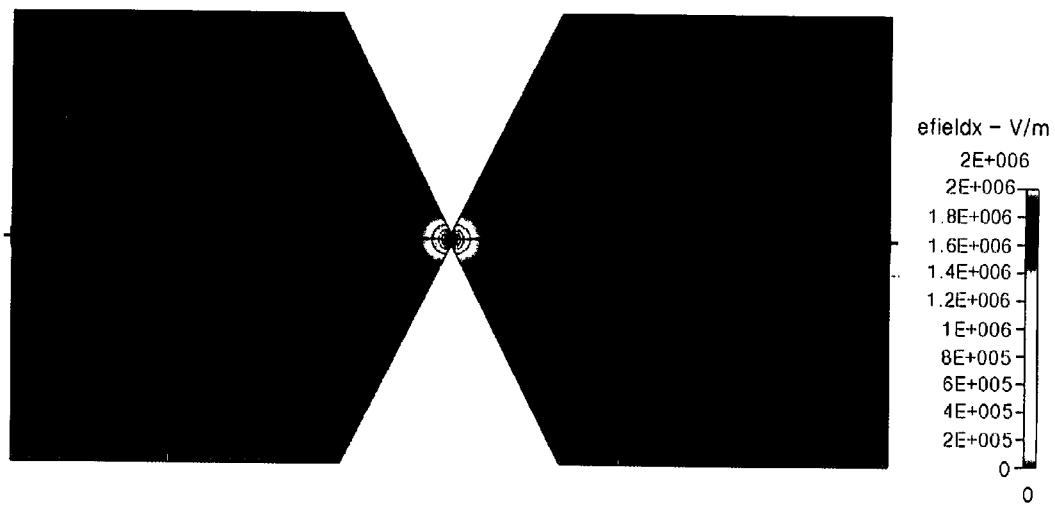
ELECTRIC FIELD (TWO-DIMENSIONAL COLUMNAR STRUCTURE)
