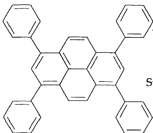
1, 3, 6, 8-tetraphenylpyrene
