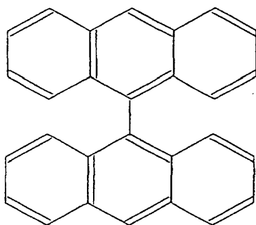
Structural formula (7)
