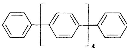
p-sexiphenyl
