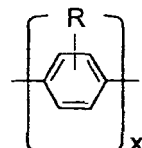
PPP derivatives
