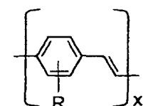
PPV derivatives
