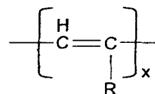
PA derivatives
