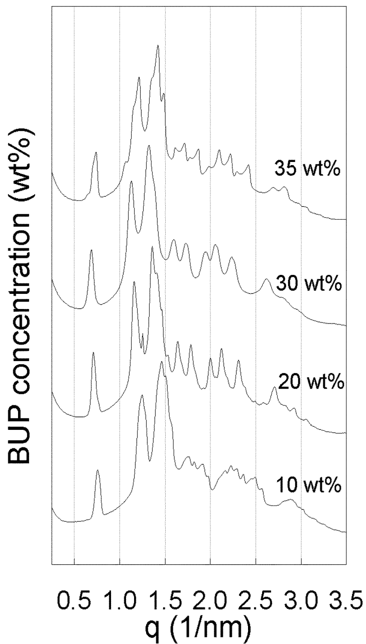
Figure. 5 X-ray diffractograms of the BJ formulations in PBS containing different amounts of BUP. Samples are prepared at formulation to PBS weight ratio of 1/9. Upon increasing BUP concentration the Fd3m liquid crystalline structure remains unchanged.
