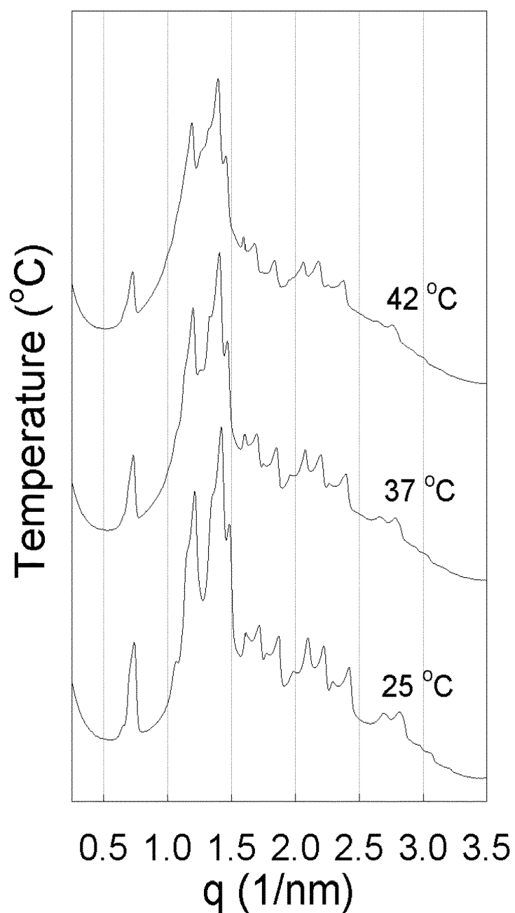
Figure. 6 X-ray diffractograms of the BJ formulation containing 35 wt% of BUP as a function of temperature. Sample is prepared at formulation to PBS weight ratio of 1/9. Upon increasing temperature from 25 to 42 °C the Fd3m liquid crystalline structure remains unchanged.
