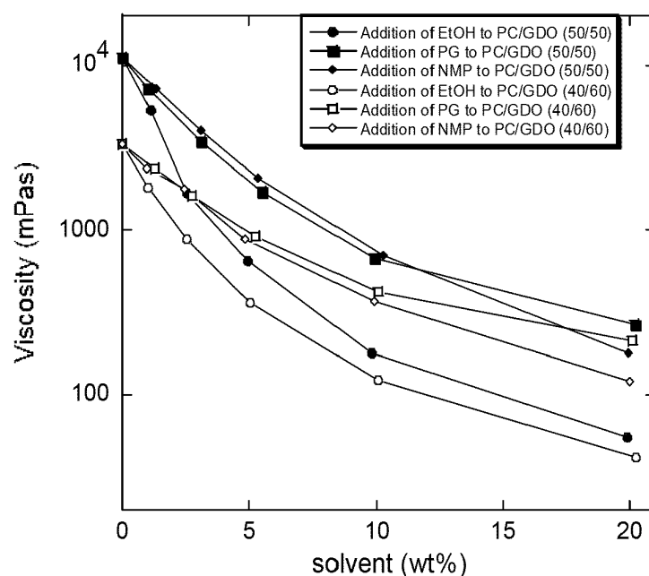
Figure 2. Decrease in viscosity at 25°C of the depot precursor on addition of solvents. PC/GDO (50/50 wt/wt) is a precursor to a reversed hexagonal H_{II} phase and PC/GDO (40/60 wt/wt) is a precursor to a reversed cubic I_2 phase.
