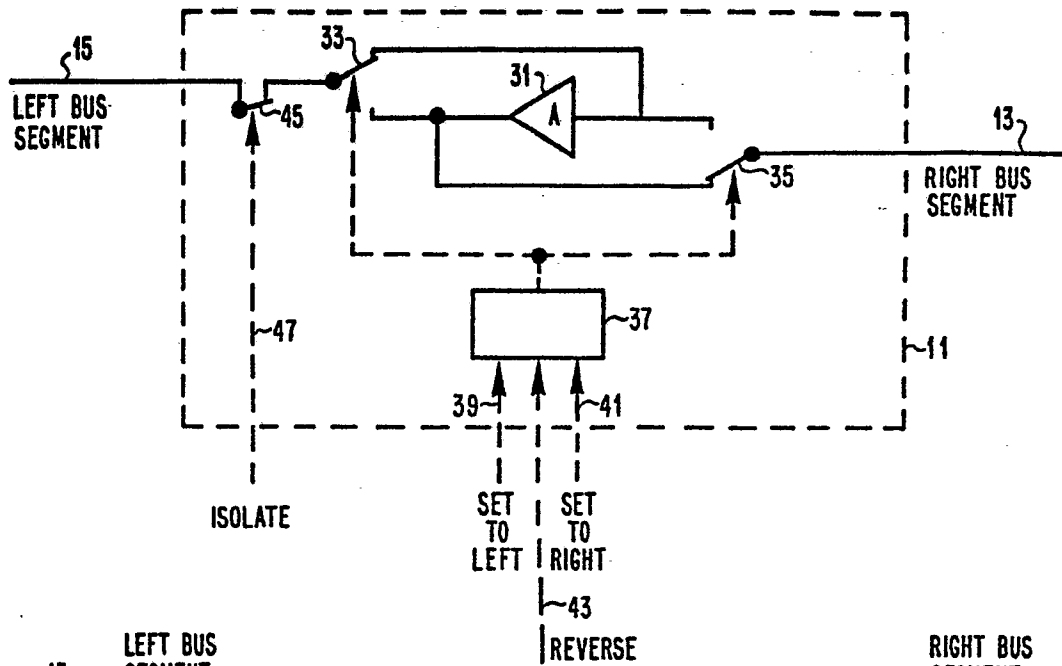
FIG. 3 SWITCH AND REPEATER UNIT
