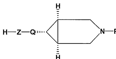
Formula X
