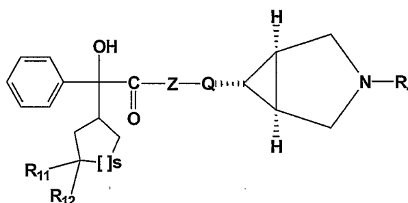
Formula IV
