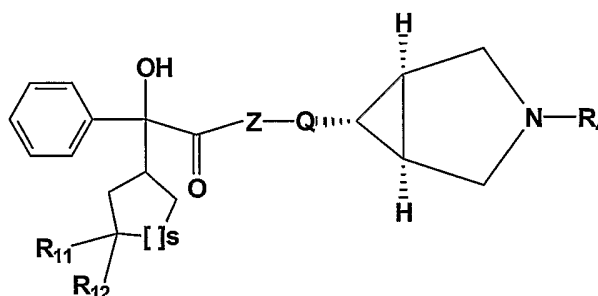
FORMULA IV
