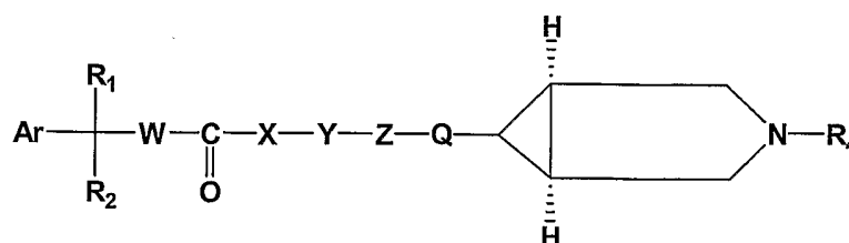
Formula II
