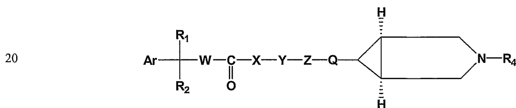
Formula II
