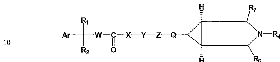
Formula I
