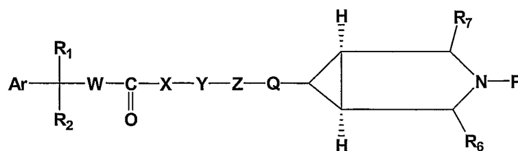
FORMULA VII
