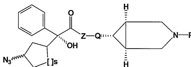
Formula XV
