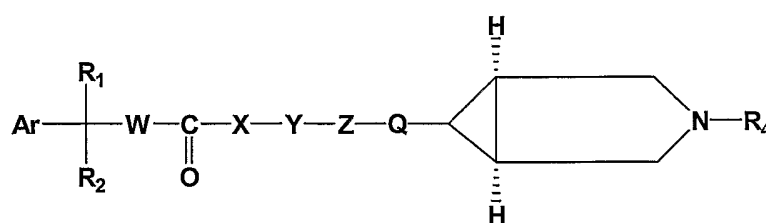
Formula II
