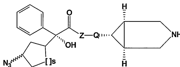
Formula XVI
