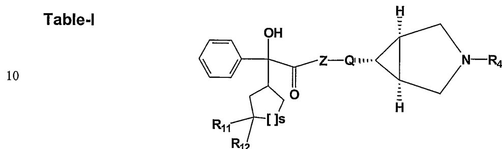
Formula – IV
