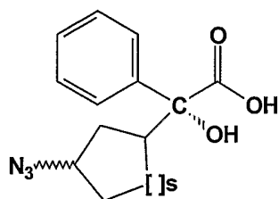
Formula XIV
