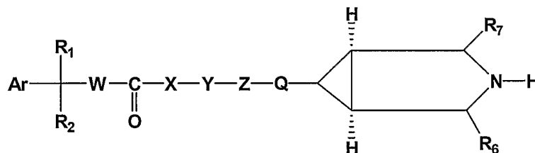
FORMULA VIII
