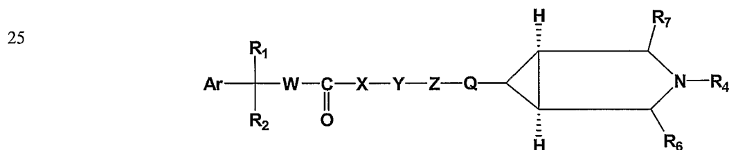
30 Formula I
