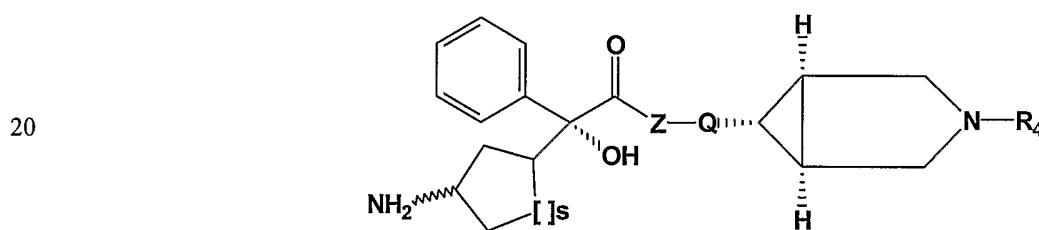
Formula XVIII
