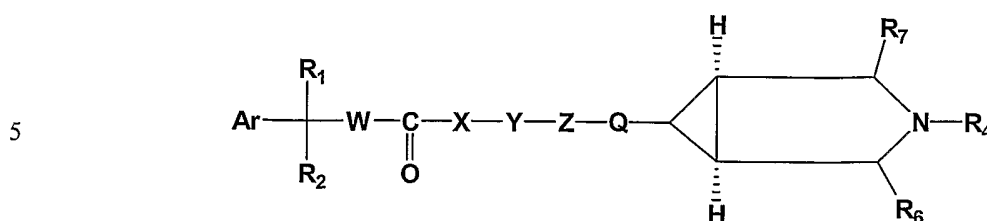
Formula I
