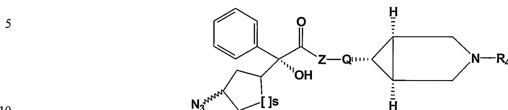
Formula XVII
