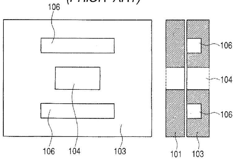
FIG. 2 (PRIOR ART)
