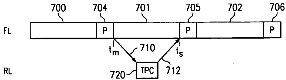
FIG. 7 (PRIOR ART)
