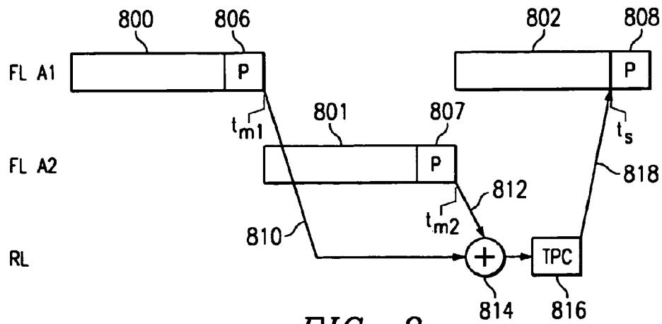
FIG. 8 (PRIOR ART)
