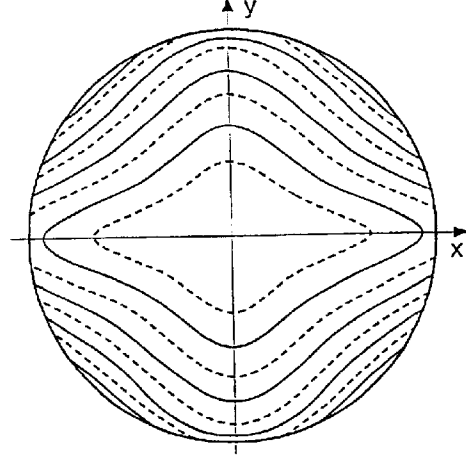
ASTIGMATISM FIRST COMPARATIVE EXAMPLE
