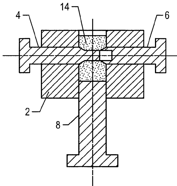
FIG. 3D
