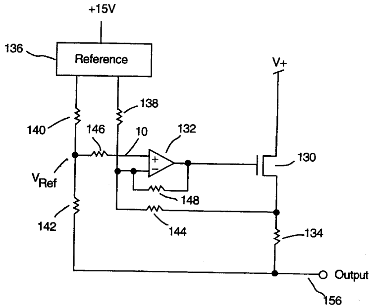
Basic Output Stage (Only Positive Half Shown)
