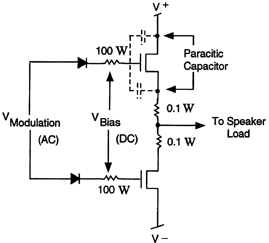
MOSFET Push-Pull Audio Output Stage
