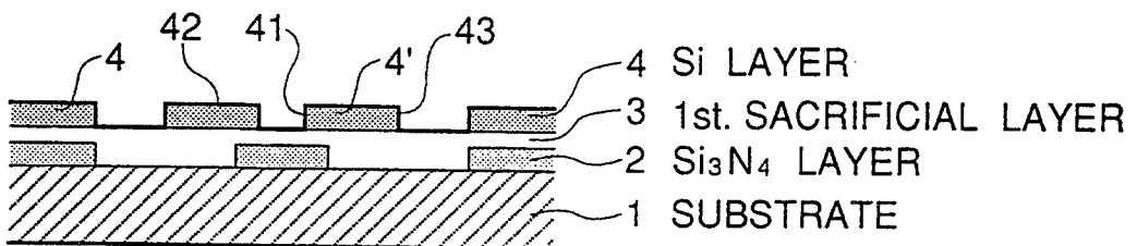
FIGURE 1E PRIOR ART
