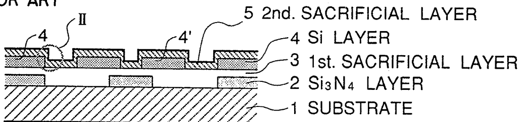
FIGURE 1F PRIOR ART
