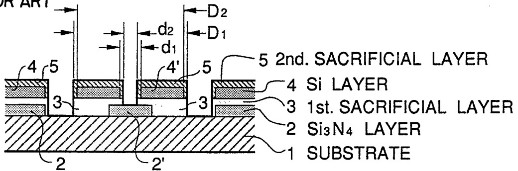
FIGURE 1H PRIOR ART
