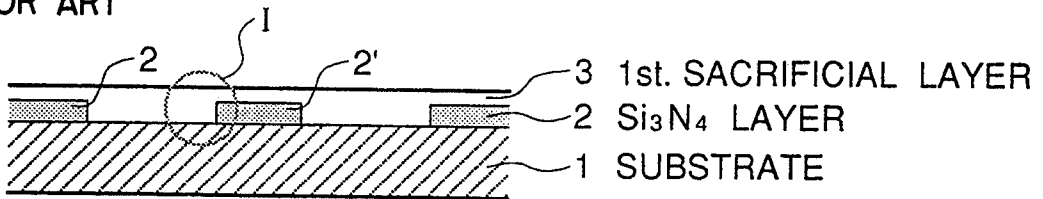
FIGURE 1D PRIOR ART
