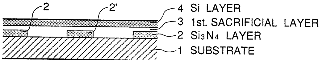
FIGURE 1E PRIOR ART
