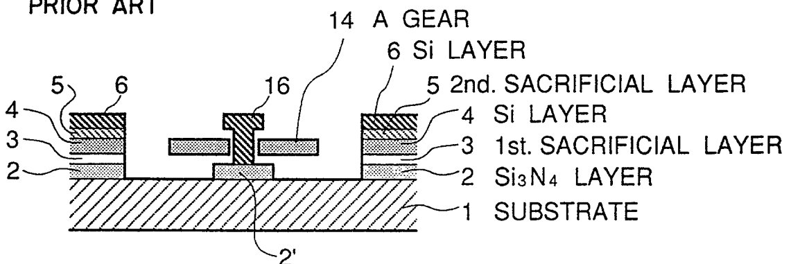
FIGURE 1J PRIOR ART
